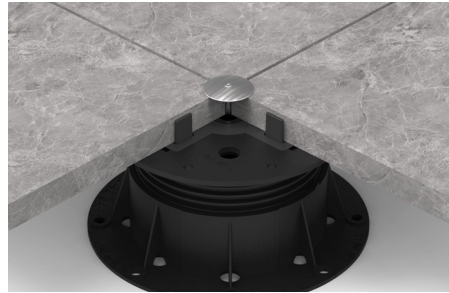
▲ WIND UPLIFT DISC USED TO SECURE LIGHTWEIGHT TILES
