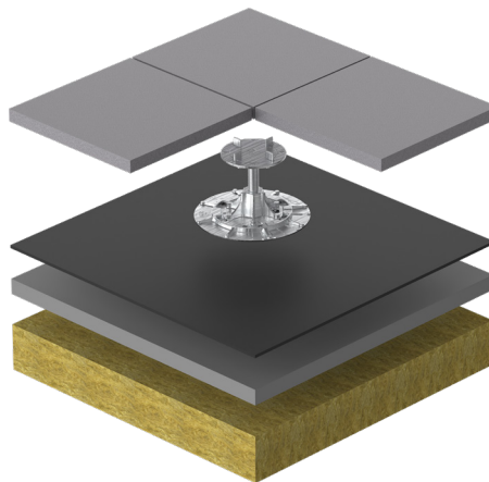
▲ OPTIONAL COVER BOARD UNDERNEATH THE WATERPROOF COVERING
